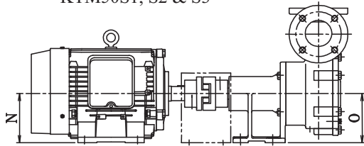
KTM50S1, S2 & S3
