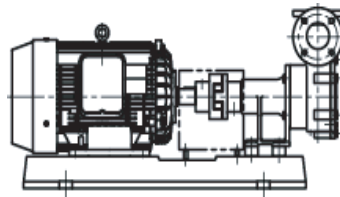
Coupling Type (Normally motor will not be supplied by NIKUNI)
