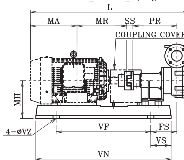
Coupling Type with Motor Dimension Model : KTM_S / KTM_F (Large Flow Rate)
