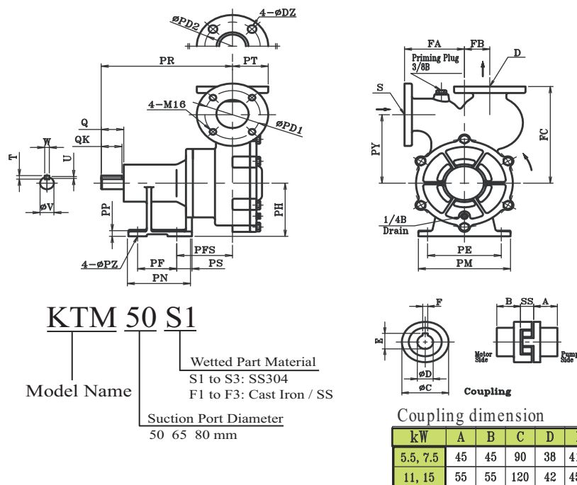
Dimension & weight Unit:mm,kg (Net weight)
