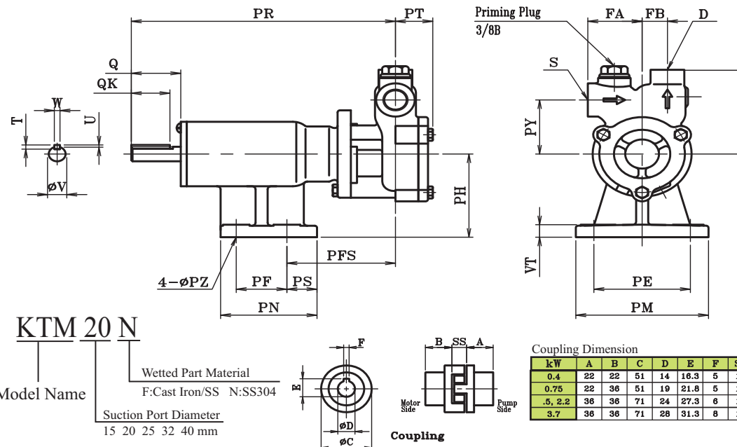
Dimension & weight
