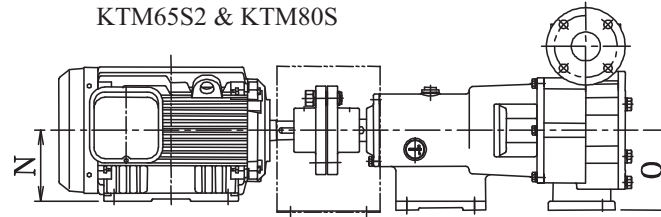
KTM65S2 & KTM80S
