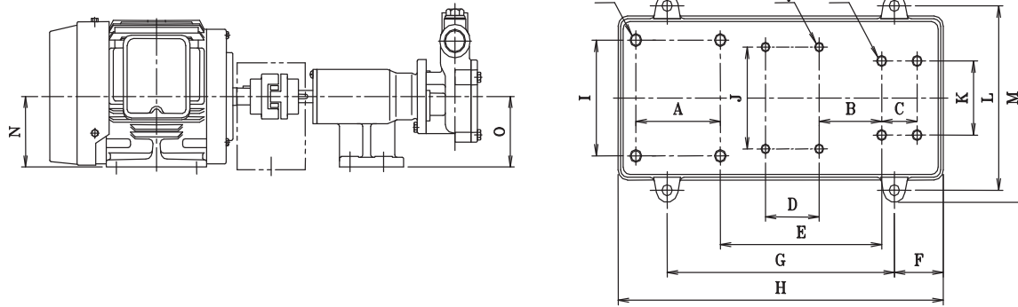
KTM50S1, S2 & S3
