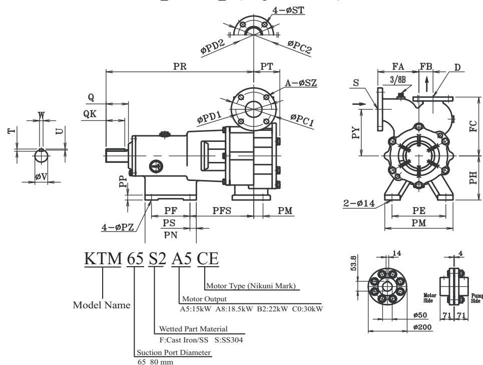
Dimension & weight Unit:mm,kg (Net weight)
