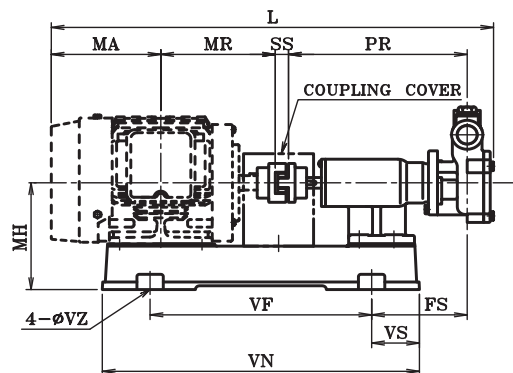
Coupling Type with Motor Dimension Model : KTM_N / KTM_F (Medium Flow Rate)
