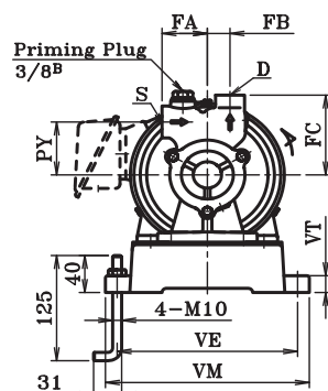
Coupling Type with Motor Dimension Model : KTM_N / KTM_F (Medium Flow Rate)
